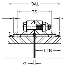
Normal Hub Arrangement
