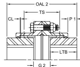
2 Hubs Reversed
