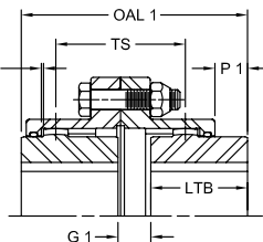
1 Hub Reversed
